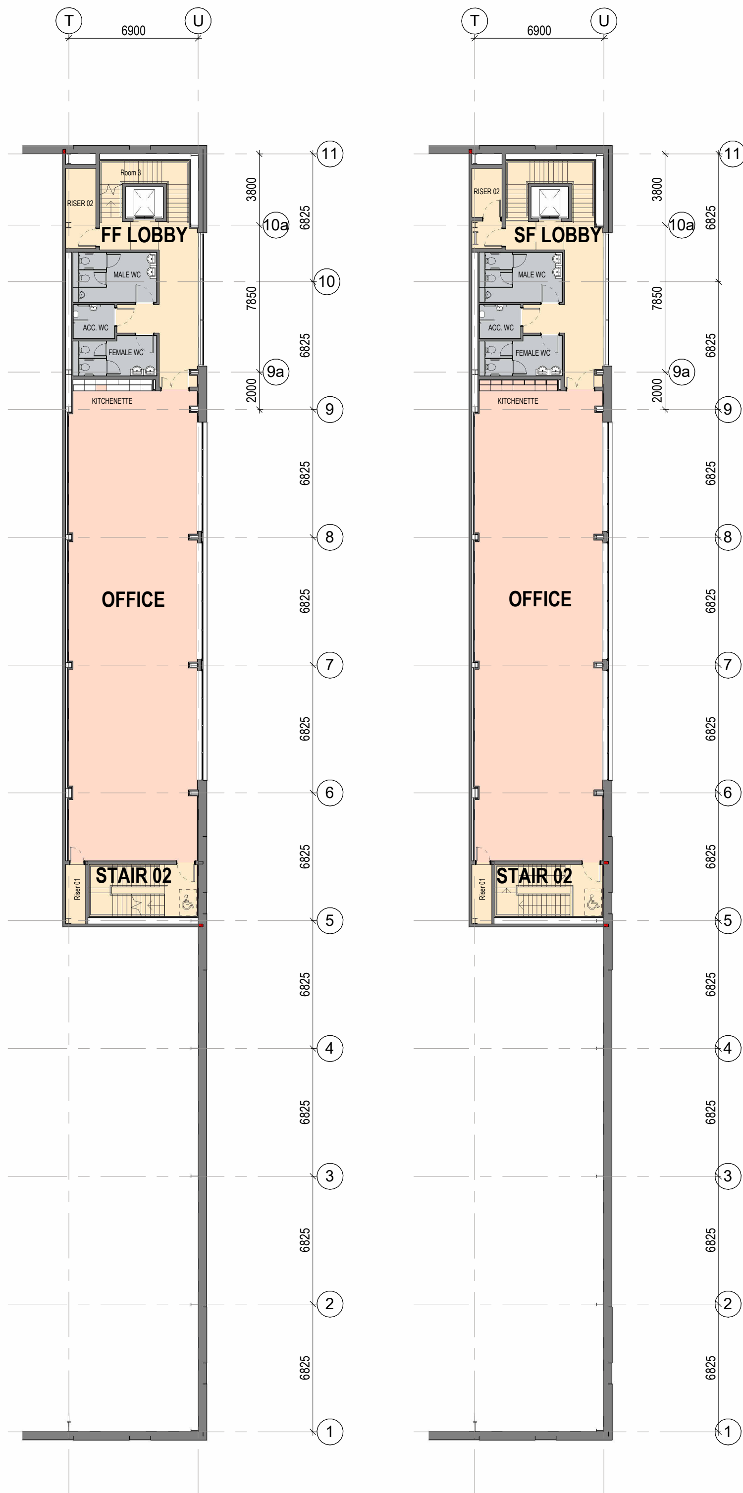
FIRST FLOOR 1 : 200
