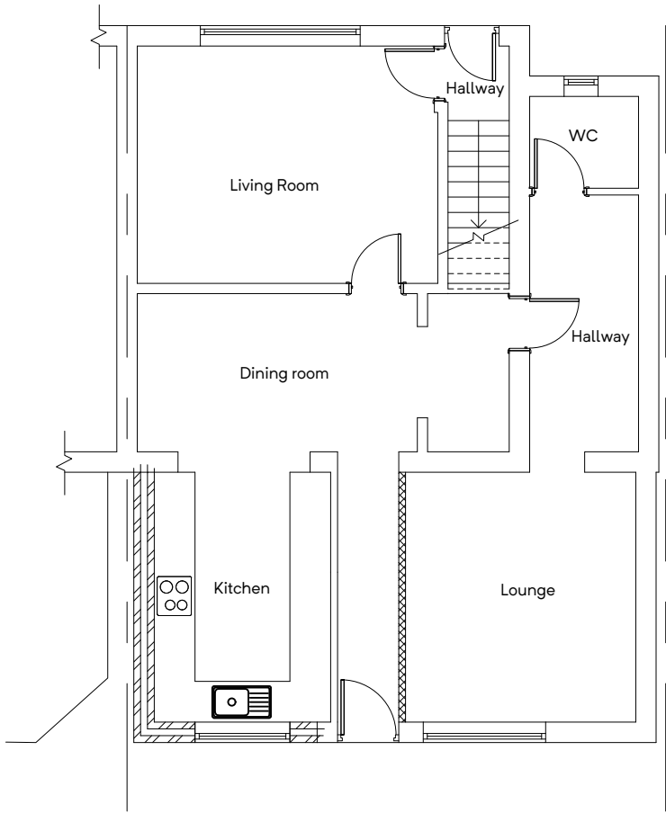
GROUND FLOOR PLAN (PROPOSED)
