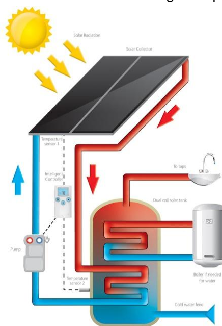
Figure 9 - The principles of a solar thermal system
