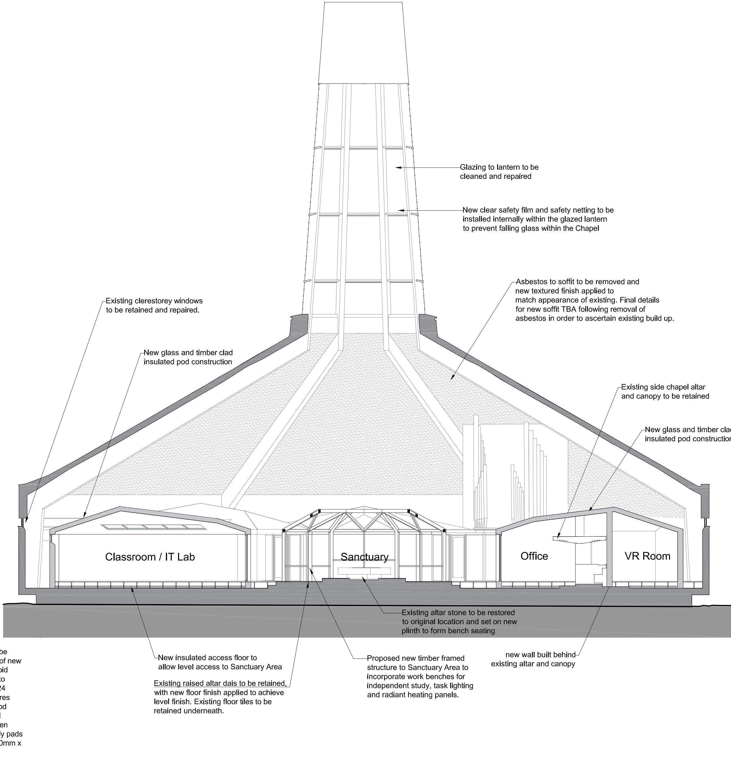
Proposed Section B
