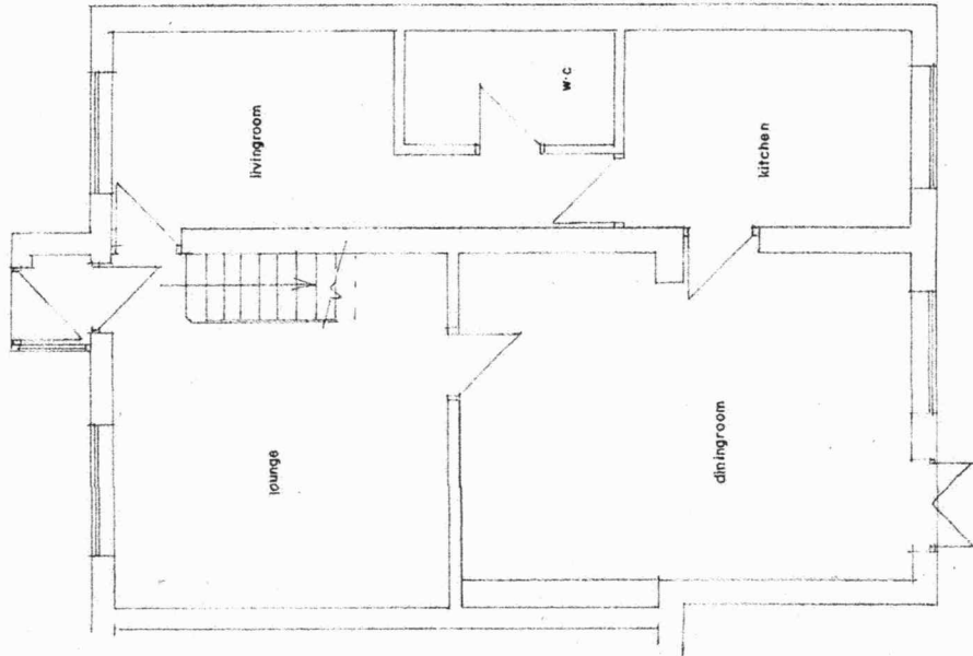
G.F. PLAN (EXISTING)
