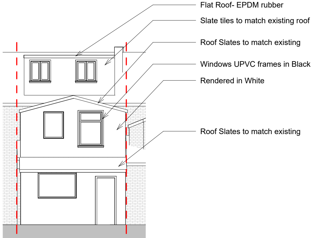
Rear Elevation as Proposed
