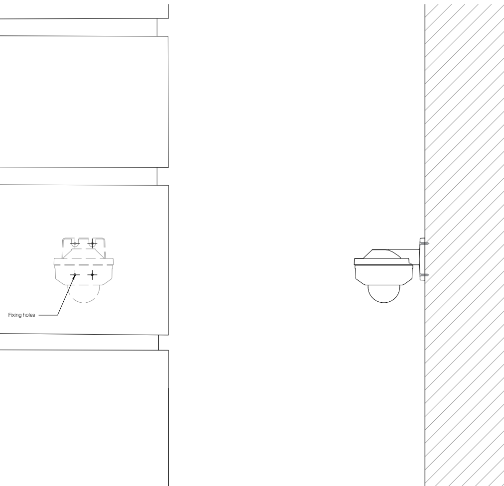
Fixing Detail 1:10@A1 / 1:20@A3
