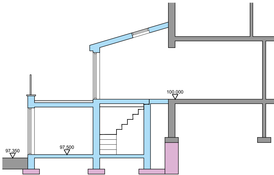
East Facing Section Through Lower Ground Floor
