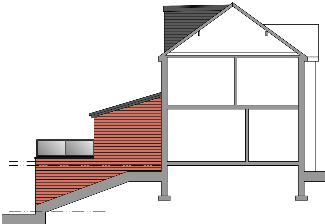
East Facing Side Elevation
