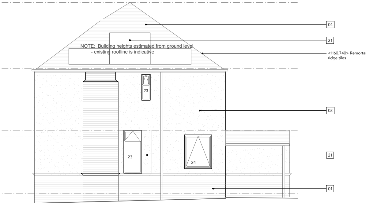
C. West Elevation
