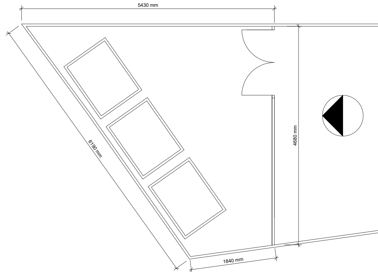
1 Detail Floor Plan _Bin Store 1:50
