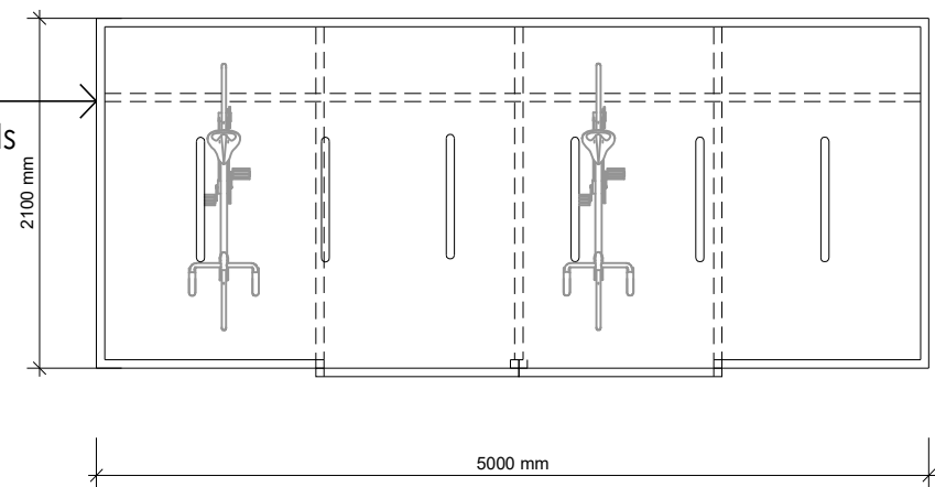
Detail Floor Plan _Bike Store 1:50
