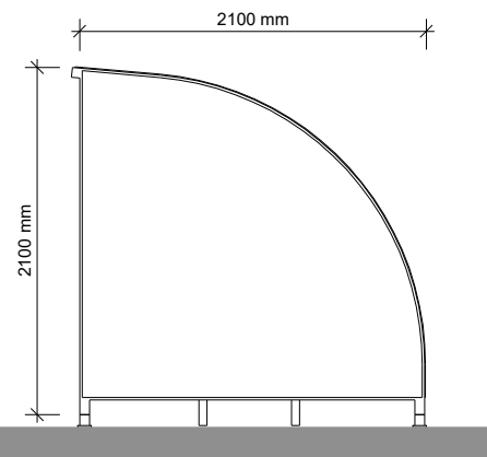
Detail Side Elevation _Bike Store 1:50
