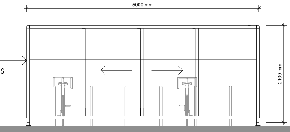
Detail Front Elevation _Bike Store 1:50
