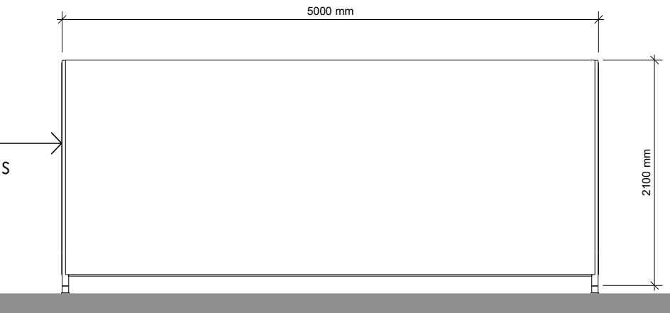
Detail Rear Elevation _Bike Store 1:50
