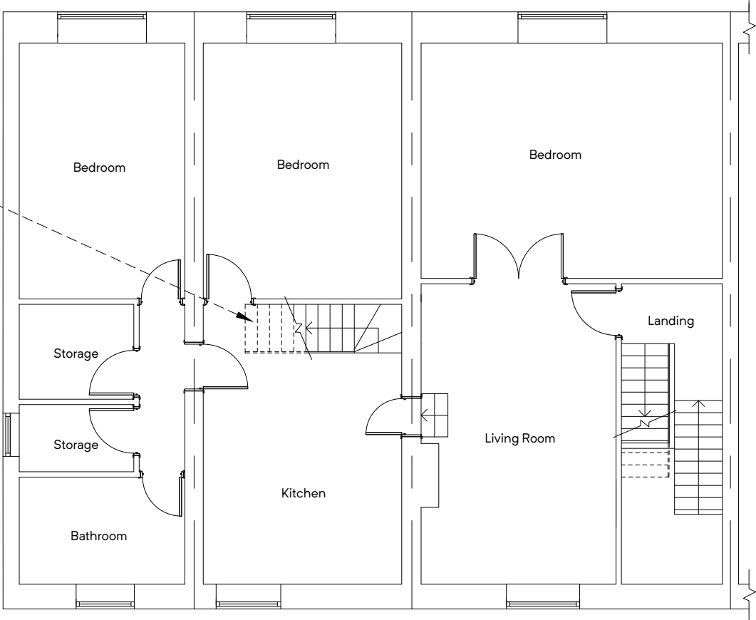
FIRST FLOOR PLAN (EXISTING)
