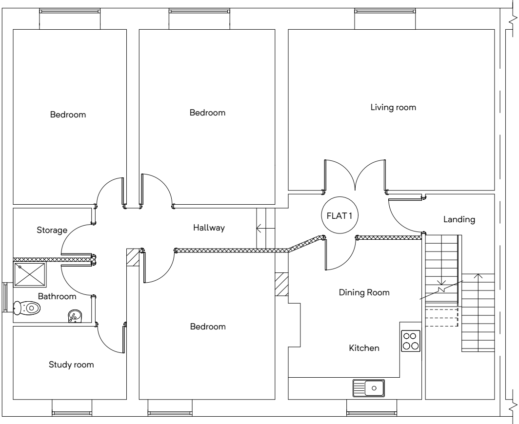
FIRST FLOOR PLAN (PROPOSED)
