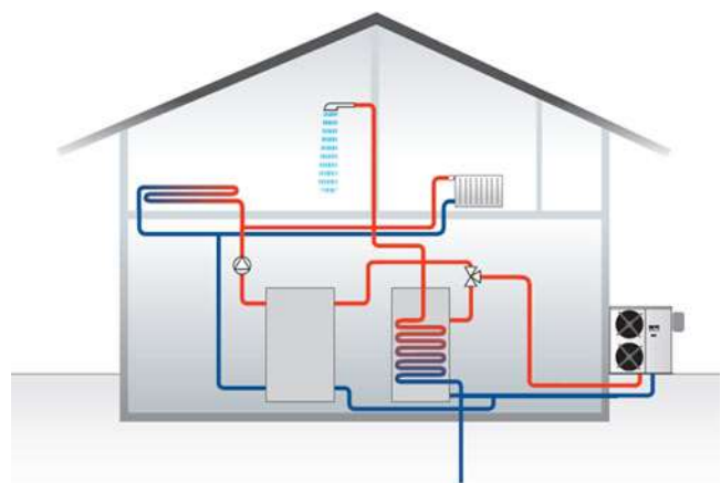
Figure 13 - Principles of an ASHP system
