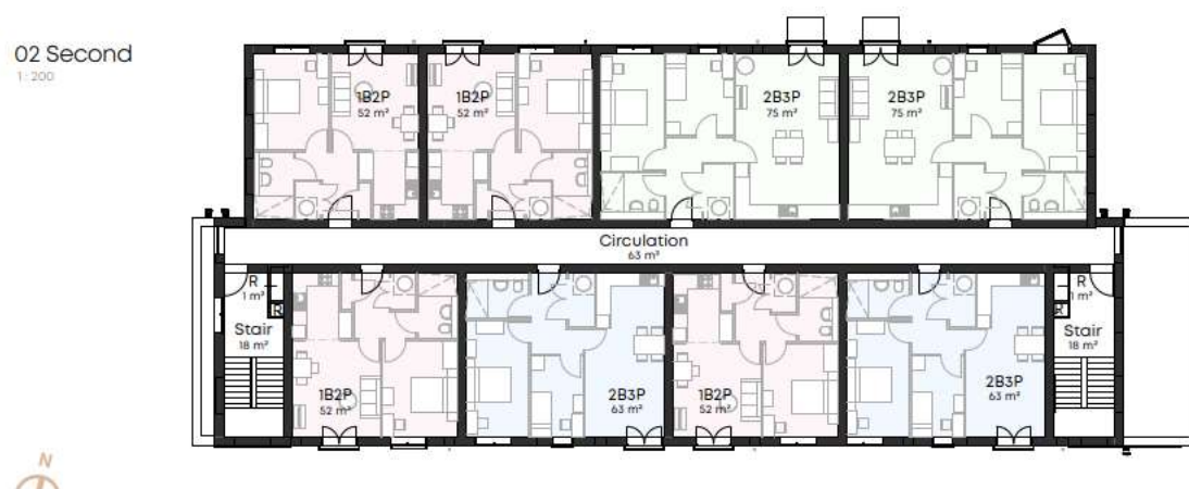
Figure 4 – Apartment's Second Floor and Roof Plan
