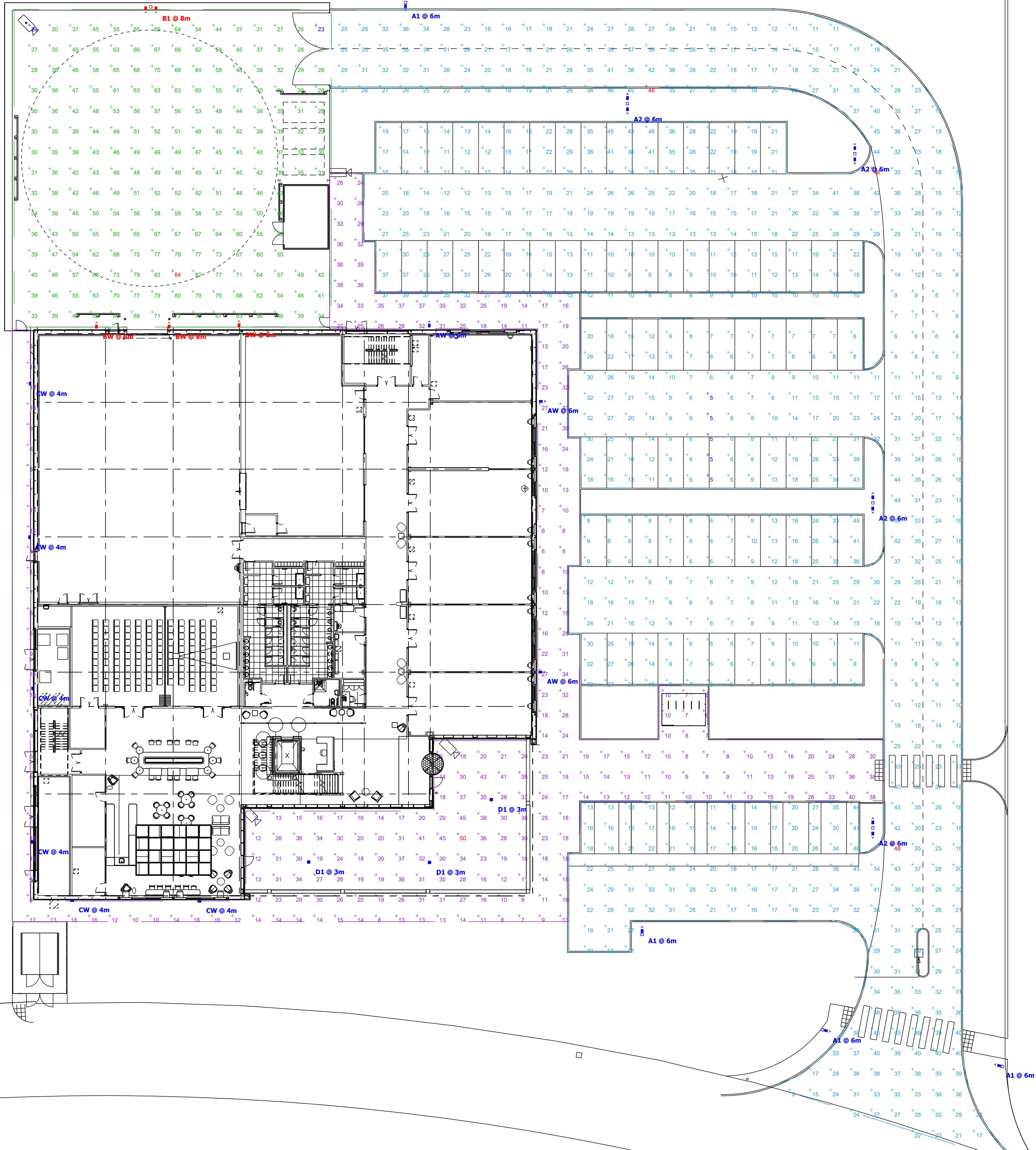
Plan View Scale - 1 : 250
