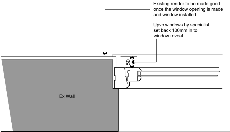
Typical plan through new window reveal Scale :- 1:10
