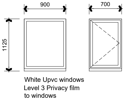
Typical Elevation to New Windows Scale :- 1:50
