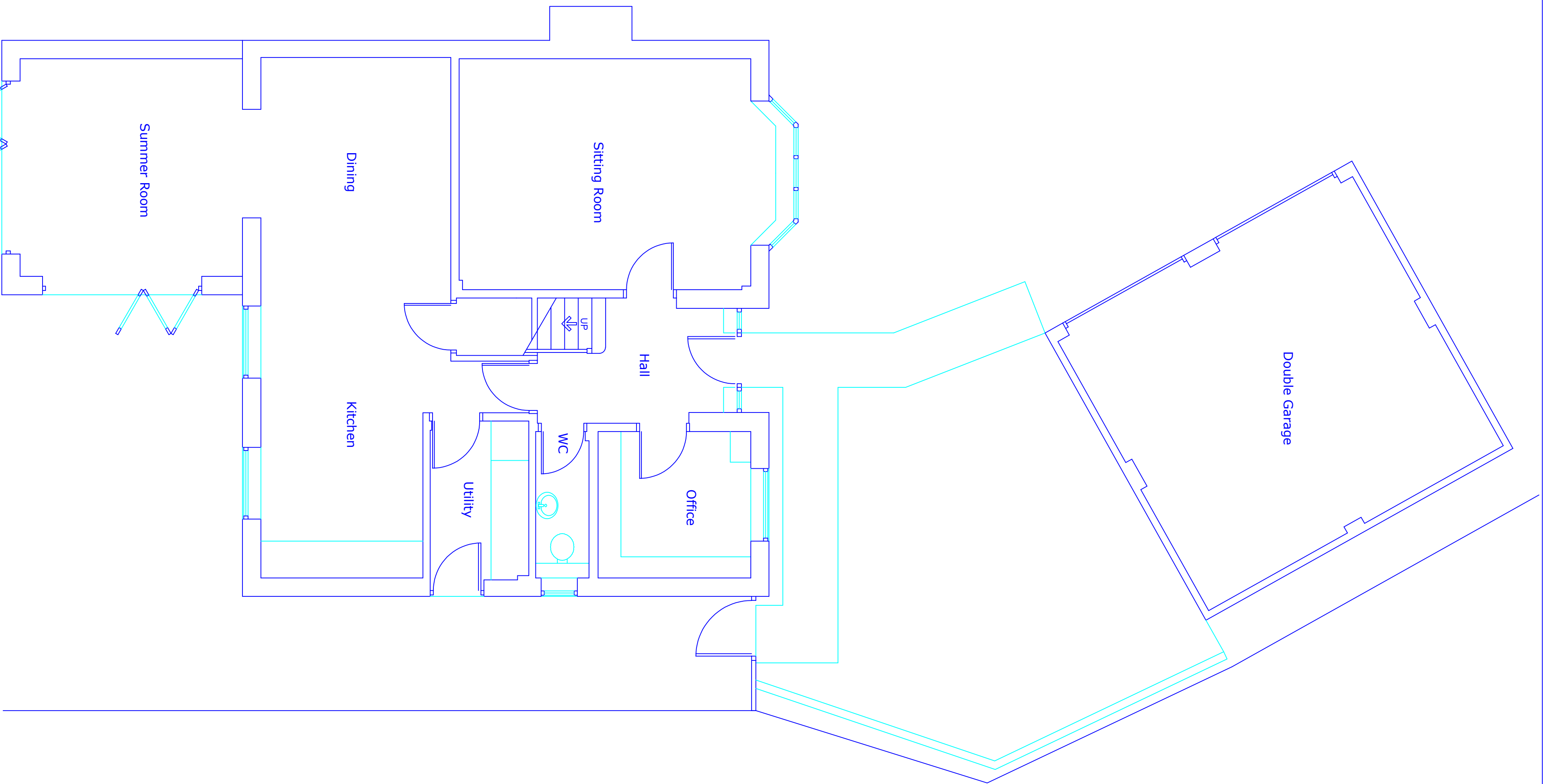
Existing Plan Ground Floor
