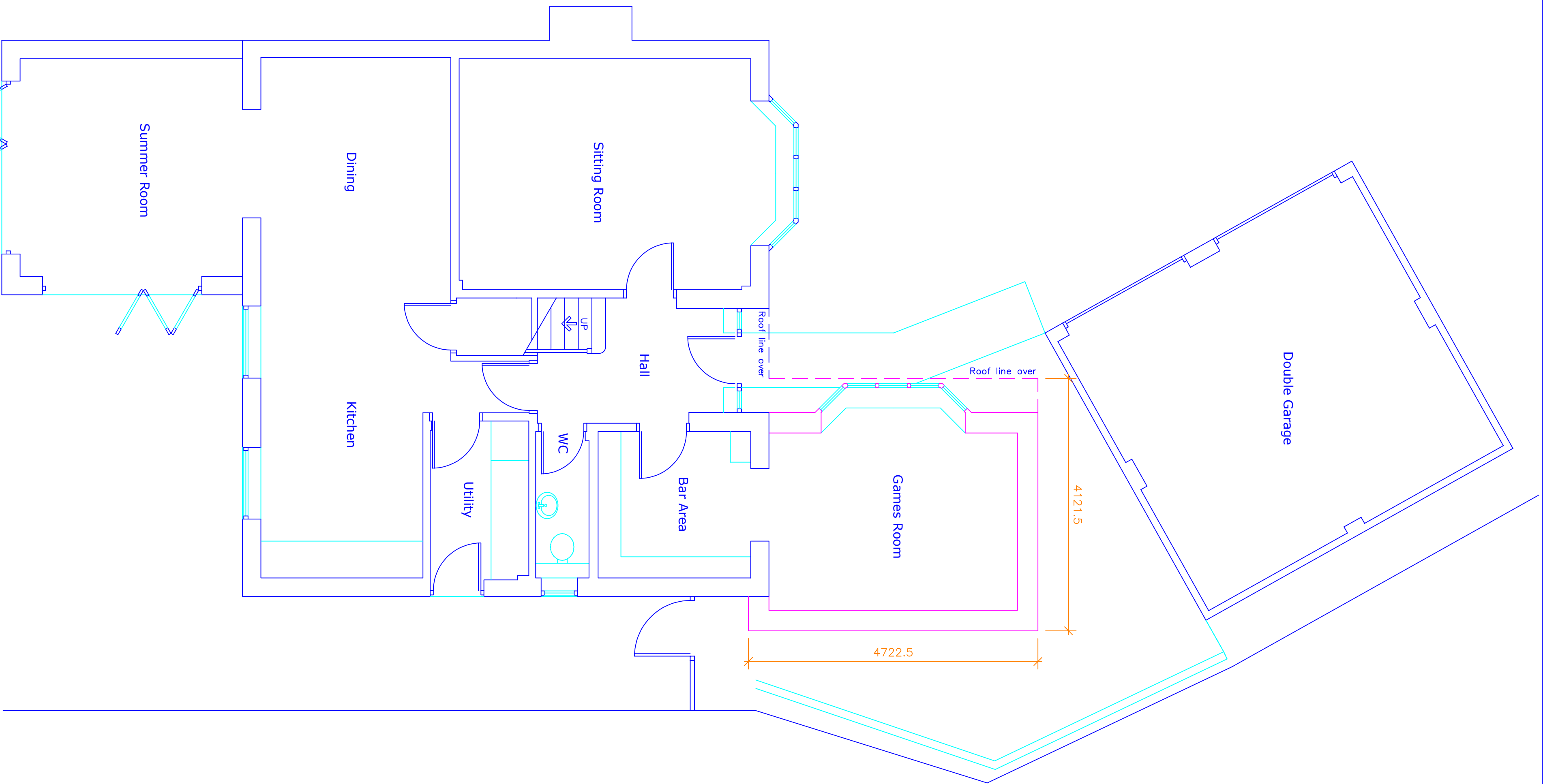
Proposed Plan Ground Floor
