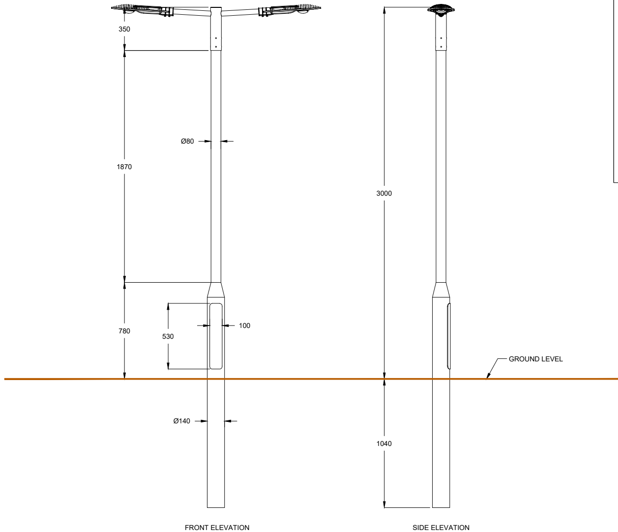
TWIN GALVANISED SIDE ENTRY LANTERN BRACKET SCALE - 1:16
