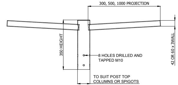
TWIN GALVANISED SIDE ENTRY LANTERN BRACKET SCALE - 1:16
