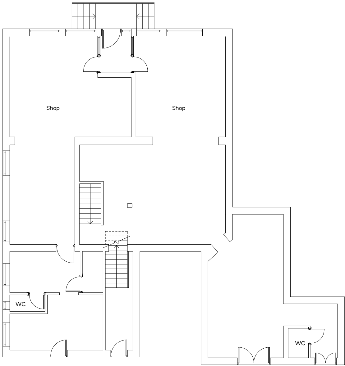
GROUND FLOOR PLAN (EXISTING)
