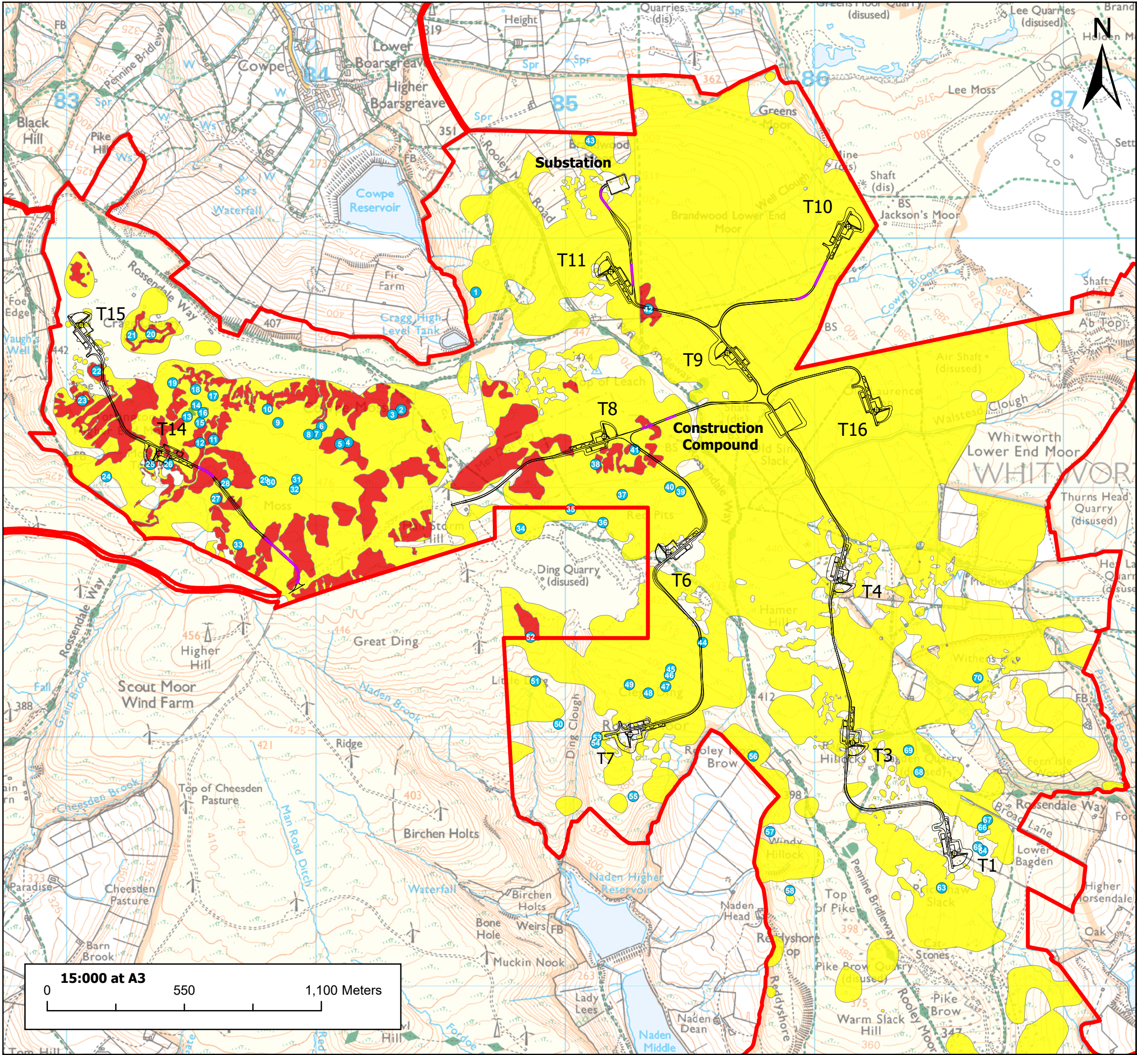
Figure 14.11: Peatland Condition Assessment
