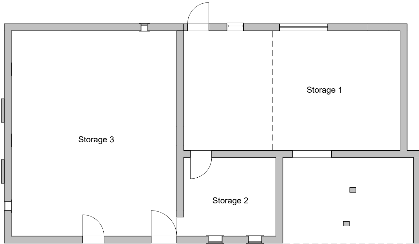
1 Ground Floor 1 : 100
