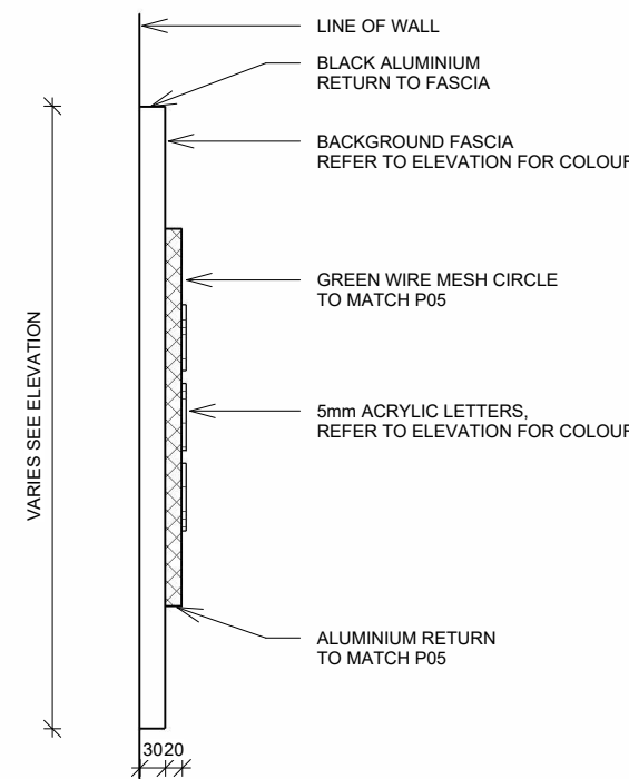
5 NON-ILLUMINATED SIGNAGE SECTION D200 1 : 10
