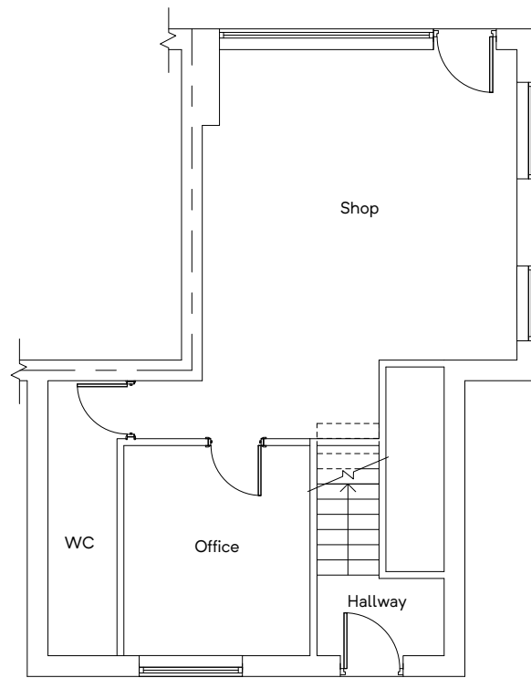
GROUND FLOOR PLAN (BEFORE & AFTER)
