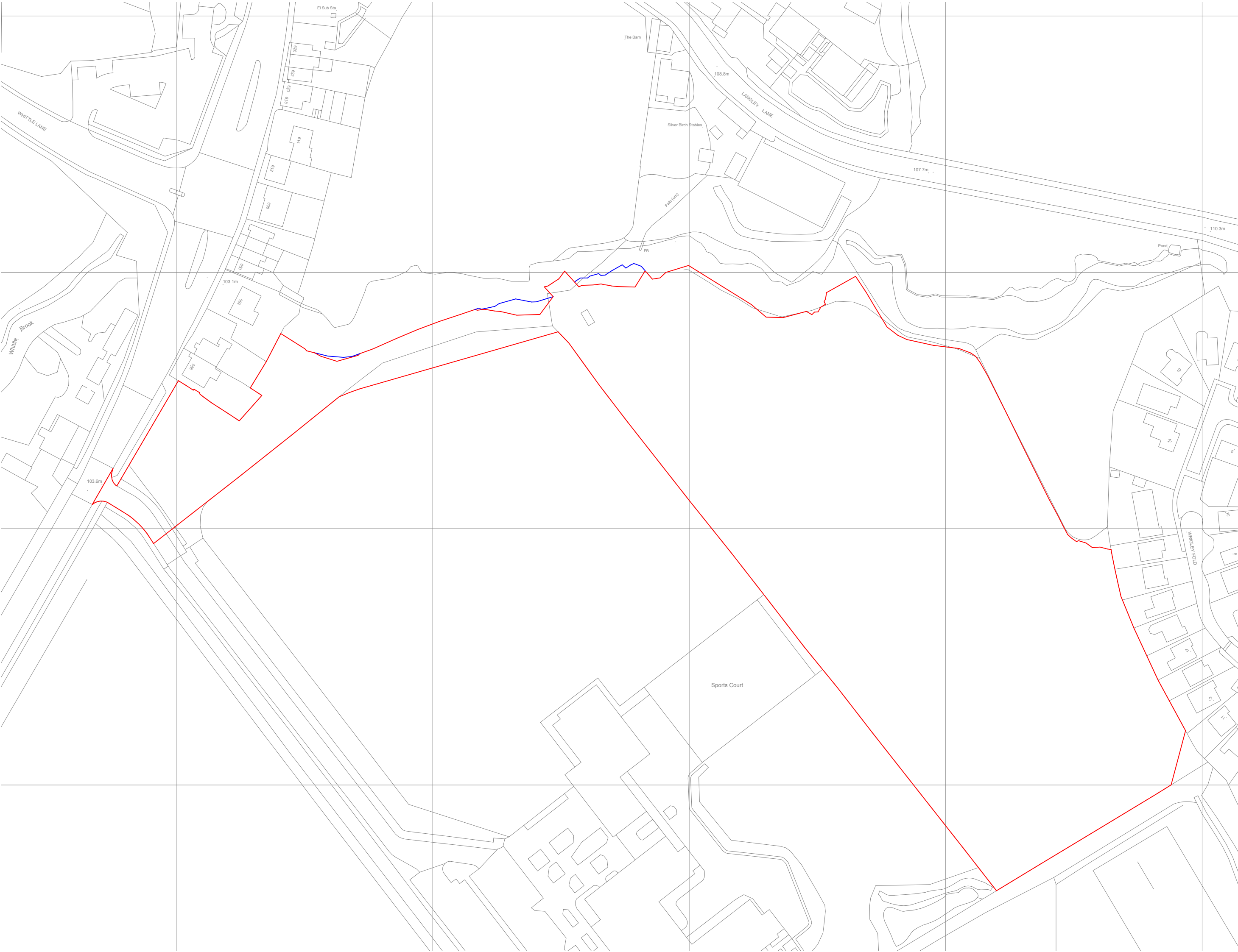
WIDER SITE LOCATION PLAN 1:1250
