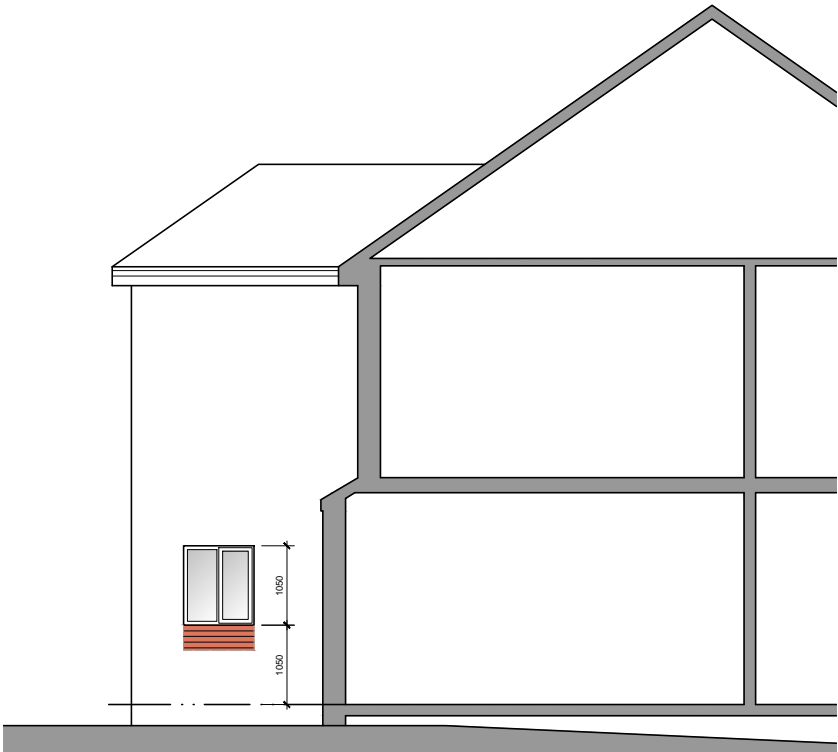
North East Facing Side Elevation
