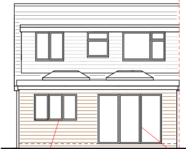
rear (southwest) elevation
