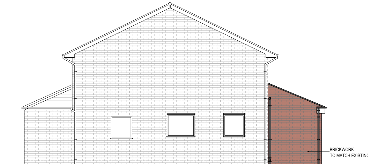
PROPOSED SIDE
