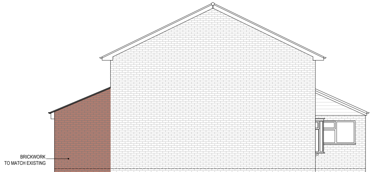
PROPOSED SIDE
