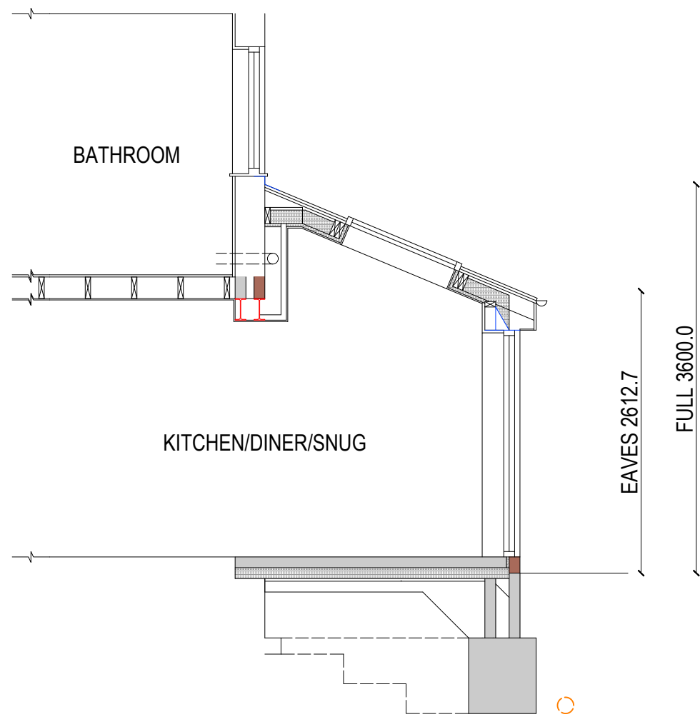
PROPOSED SECTION A-A
