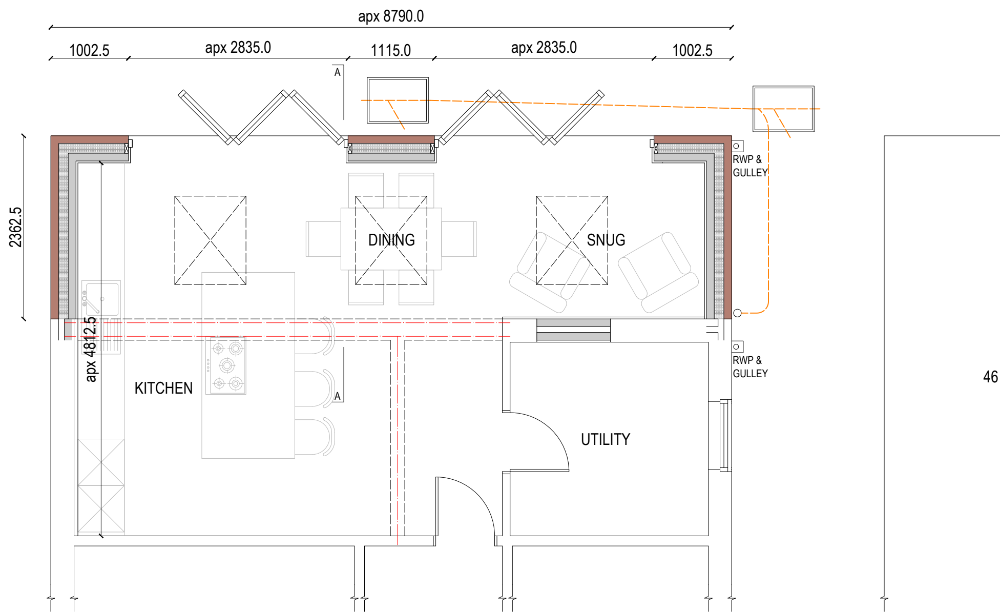
PROPOSED GROUND
