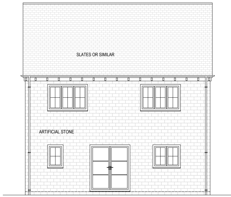
EXISTING REAR
