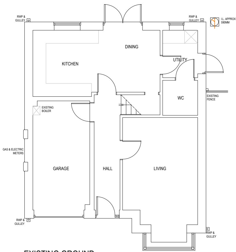
EXISTING GROUND
