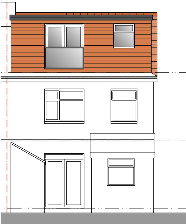
West Facing Rear Elevation
