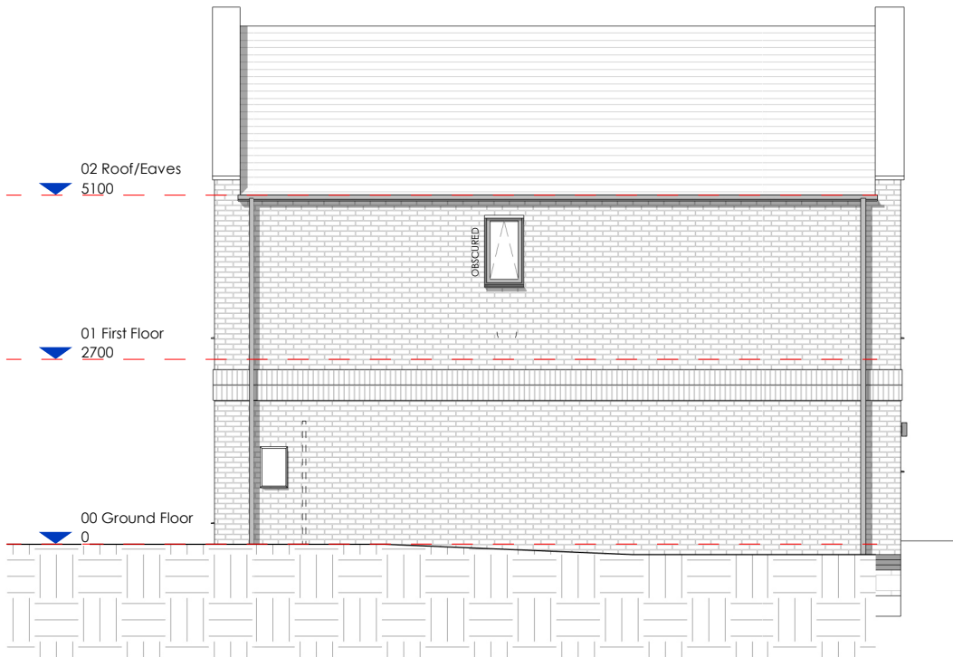
04 Elevation - Right Side 1 : 100
