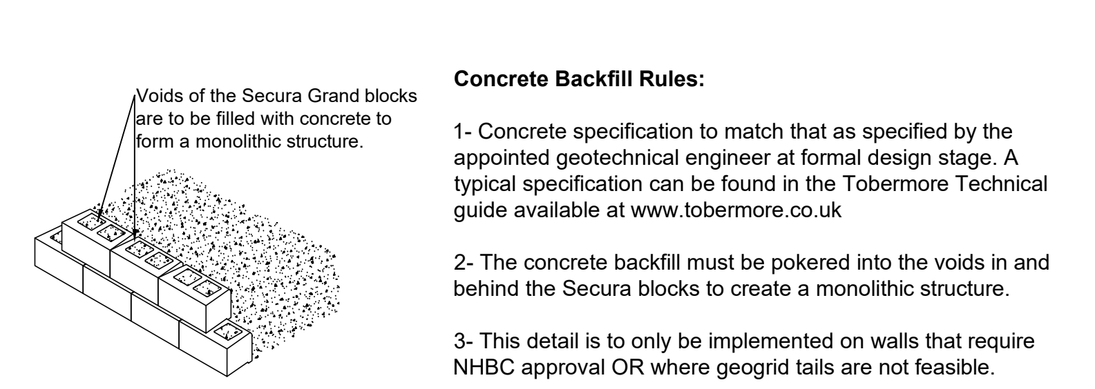
NHBC Concrete Infill Detail:
