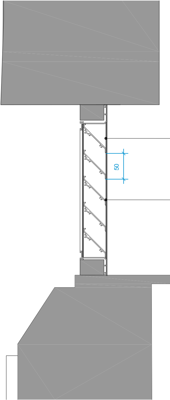
Typical Proposed External Louvre Section
