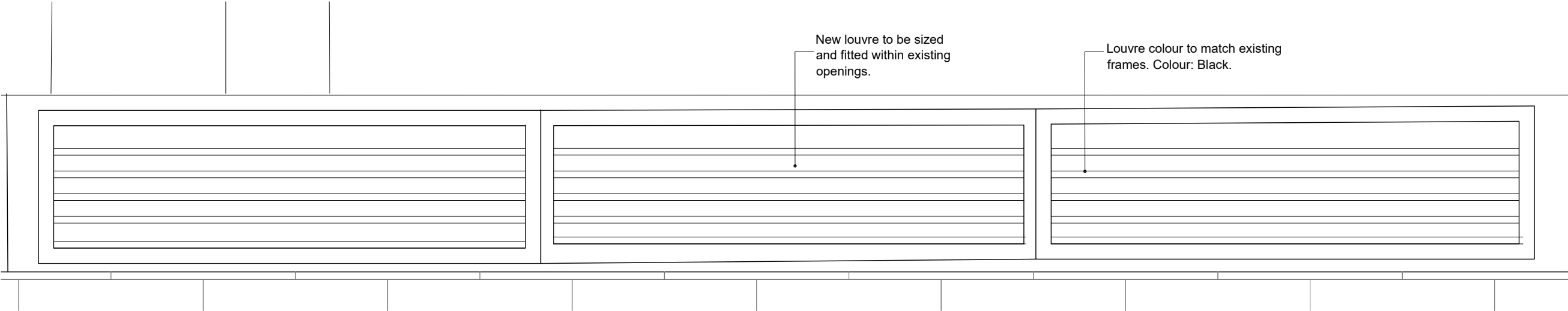
Typical Proposed External Louvre Elevation
