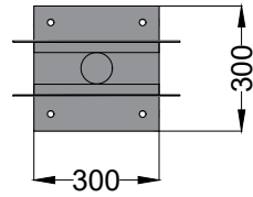
C Totem - Plan View
