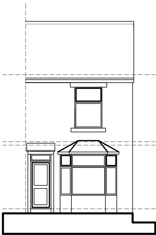
EXISTING FRONT ELEVATION 1:100
