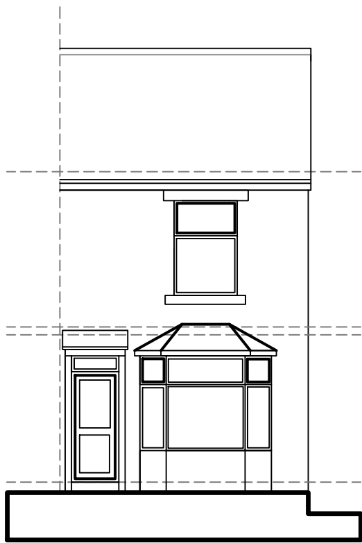
PROPOSED FRONT ELEVATION 1:100
