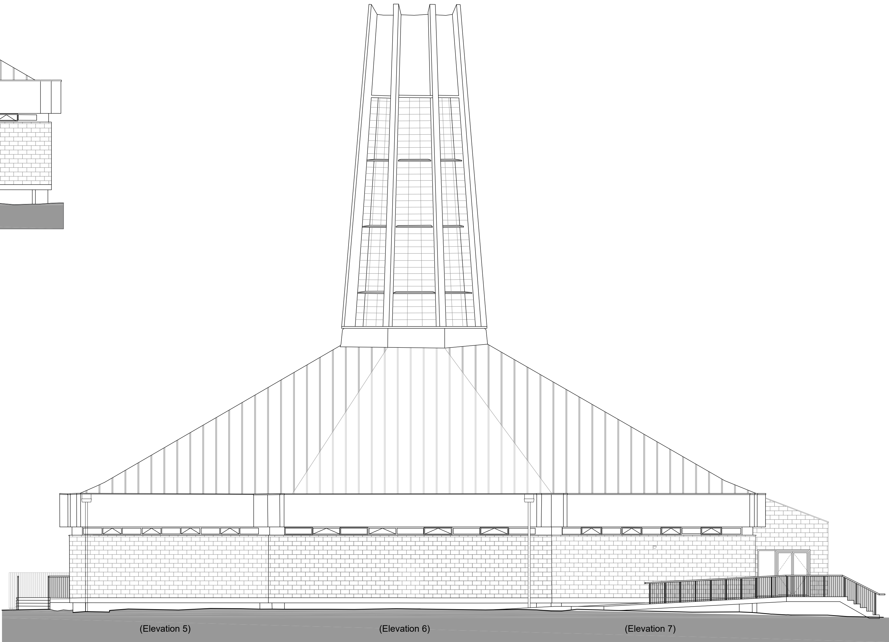
Elevation C
