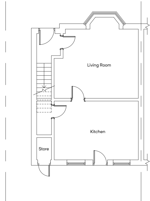
GROUND FLOOR PLAN (EXISTING)
