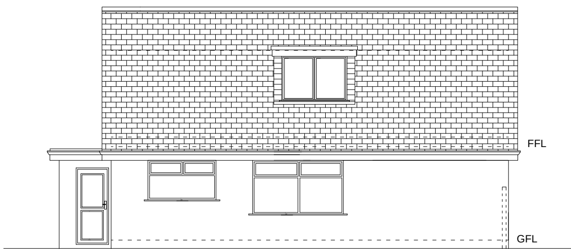
Existing LHS Elevation
