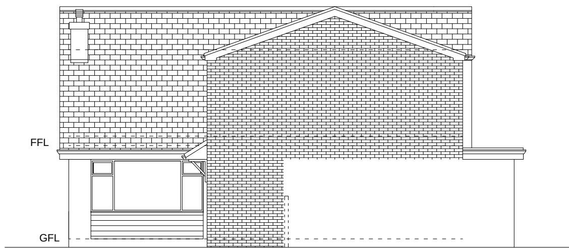
Proposed RHS Elevation
