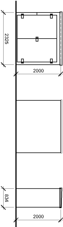
Front Elevation Rear Elevation Side Elevation Scale 1:100 Scale 1:100 Scale 1:100
