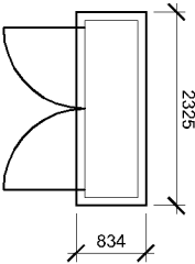
Floor Plan Scale 1:100
