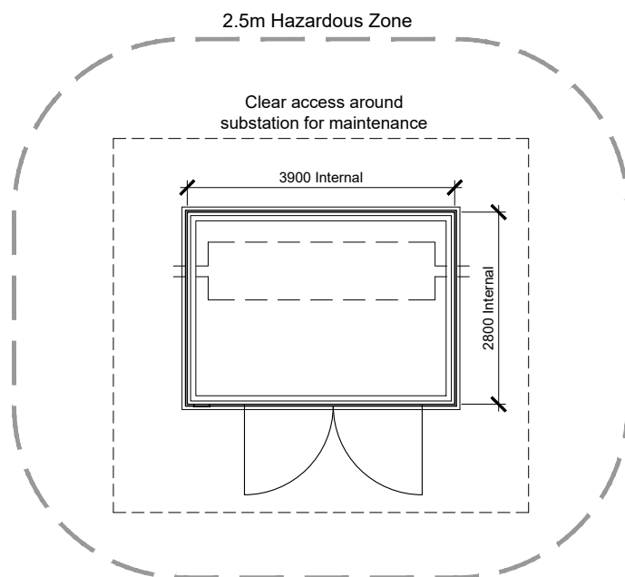
Floor Plan
