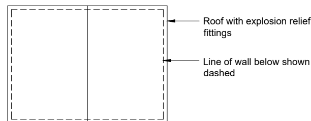
Roof Plan
