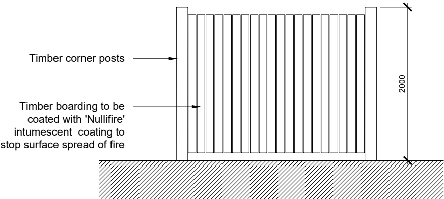
Rear Elevation
