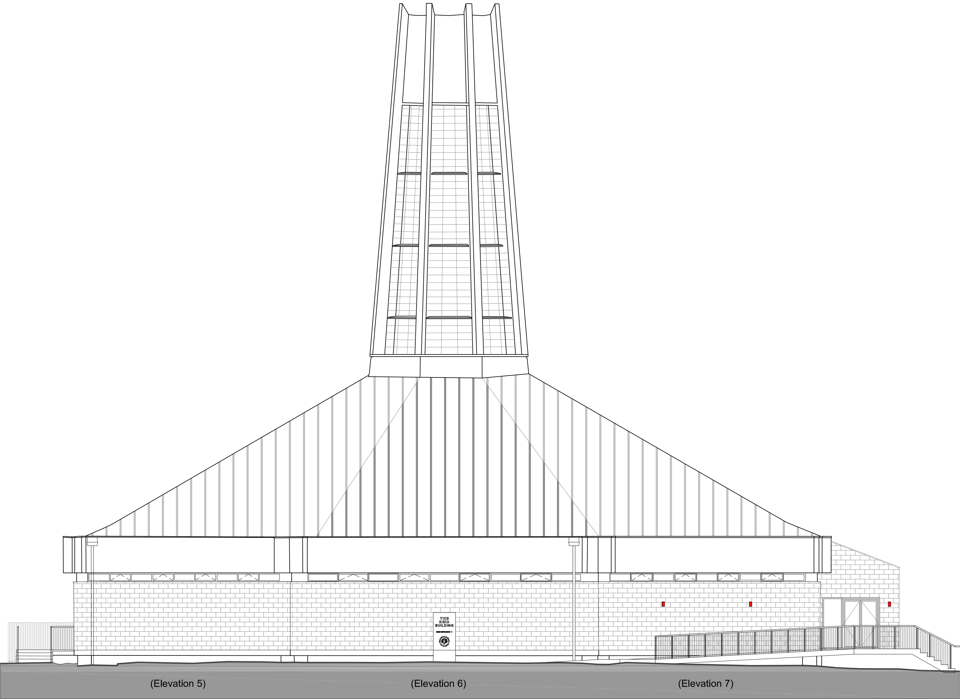
Elevation C
