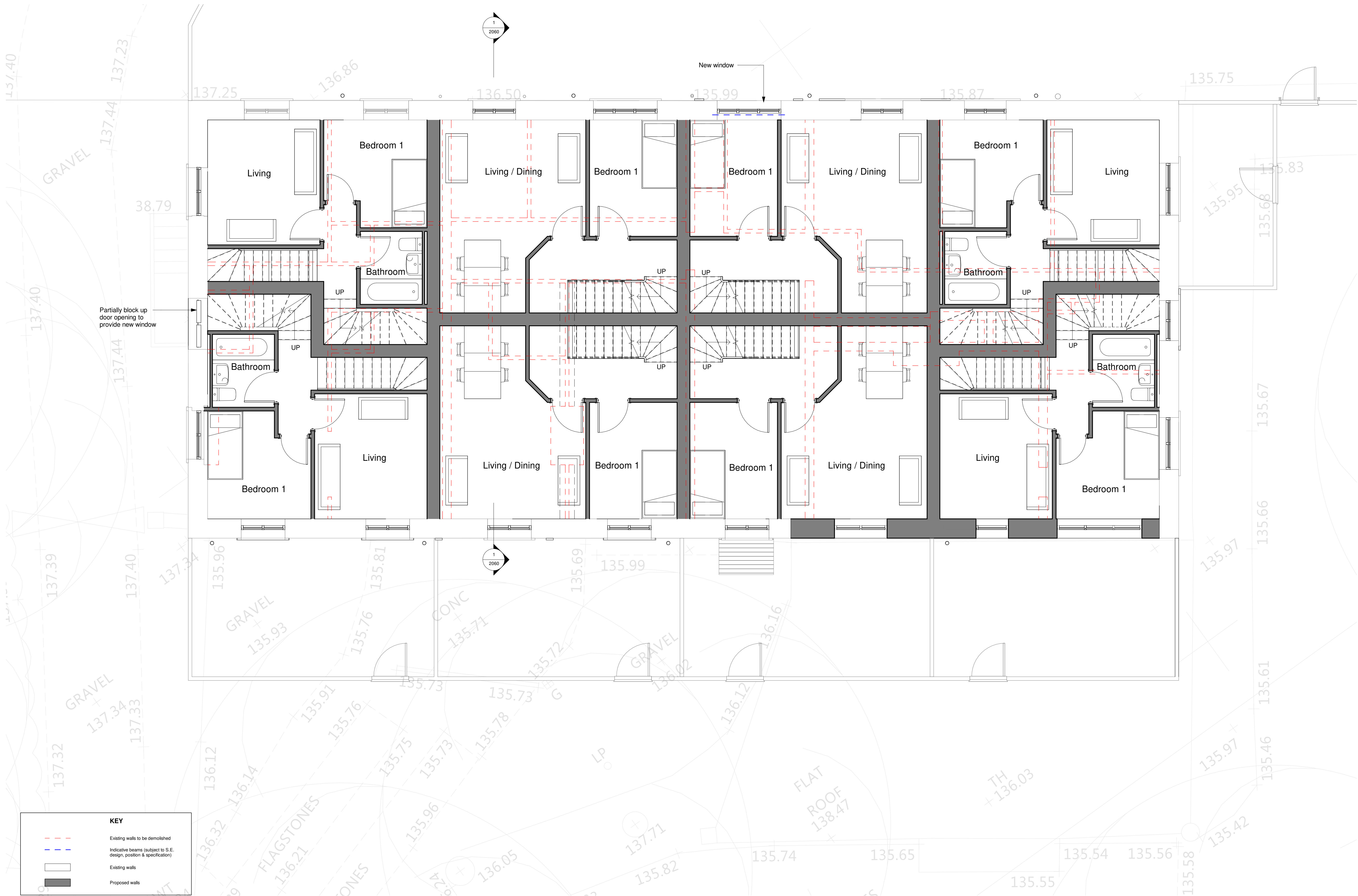
1 Proposed Level 1 1 : 50
