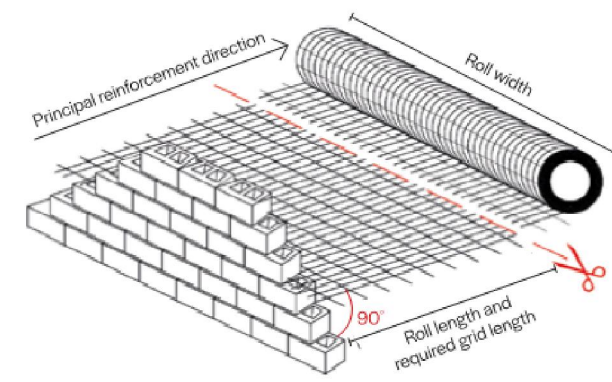
GEOGRID INSTALLATION DETAIL
