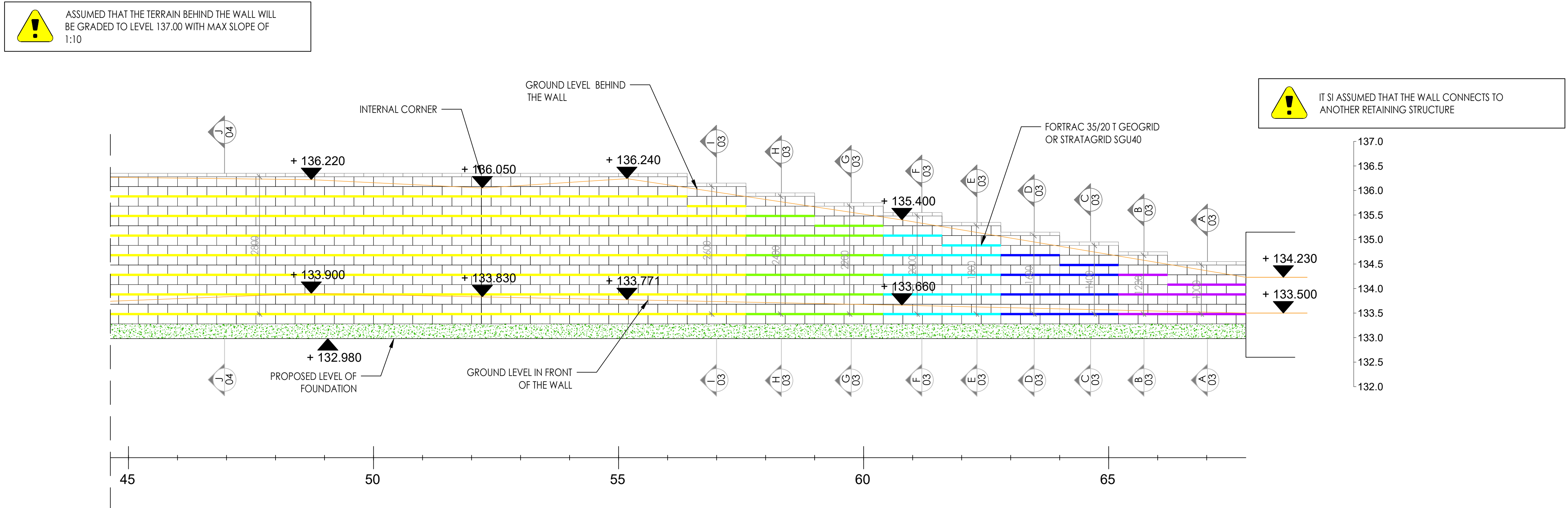
ELEVATION WALL 1-2 Scale 1:50
