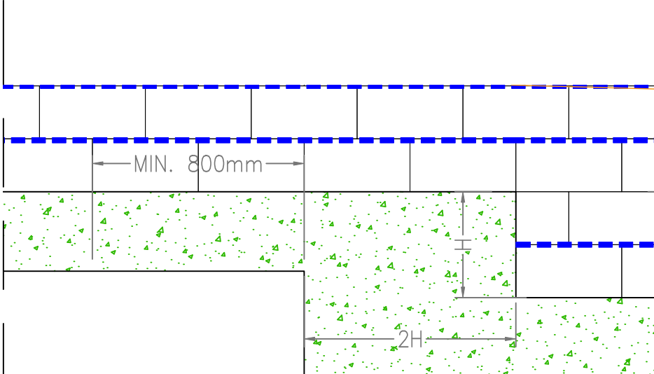
DETAIL A Scale 1:20
