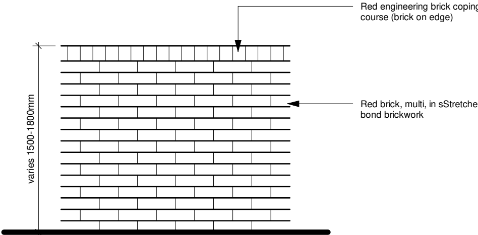
Brick Enclosure Elevation
