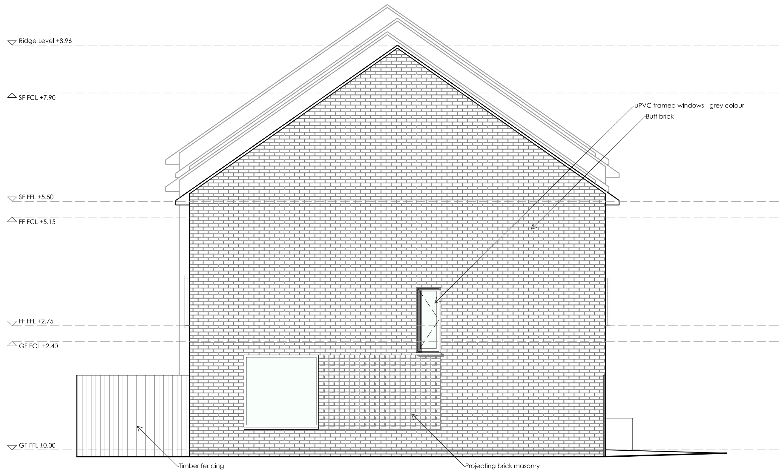
Side Elevation
