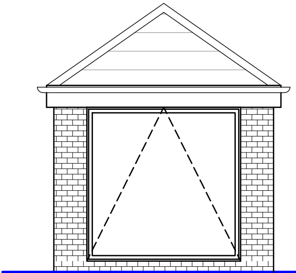
OUTBUILDING B PROPOSED REAR ELEVATION
