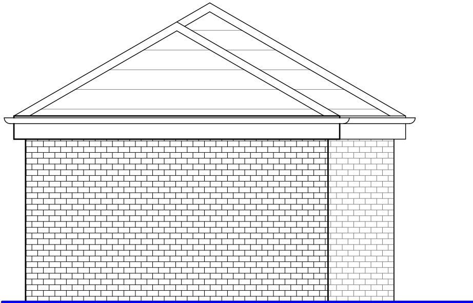
OUTBUILDING A PROPOSED SIDE ELEVATION
