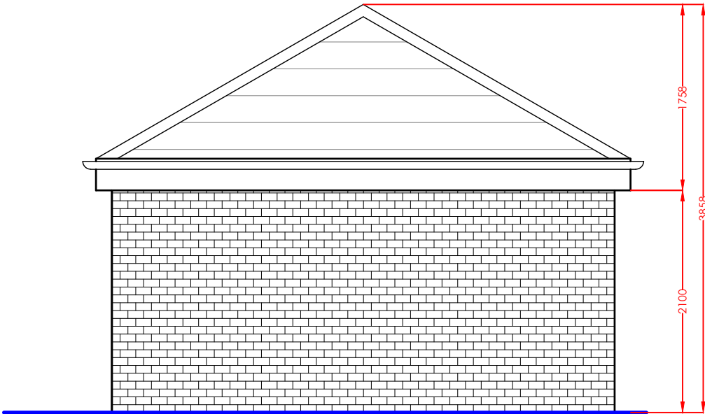
OUTBUILDING A PROPOSED SIDE ELEVATION
