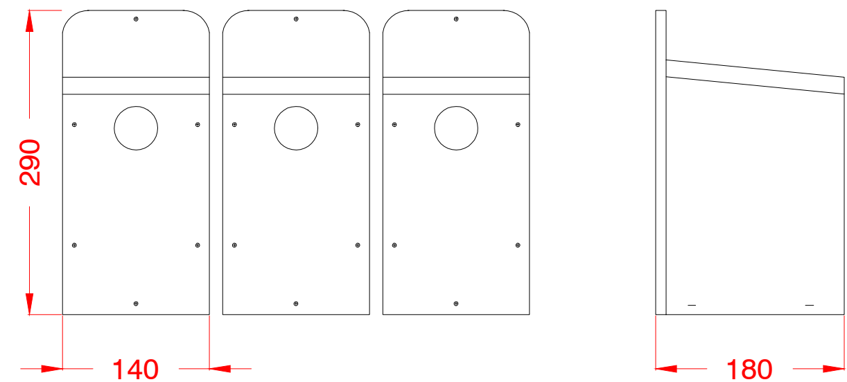
BIRD BOX FRONT ELEVATION Scale: 1:5
