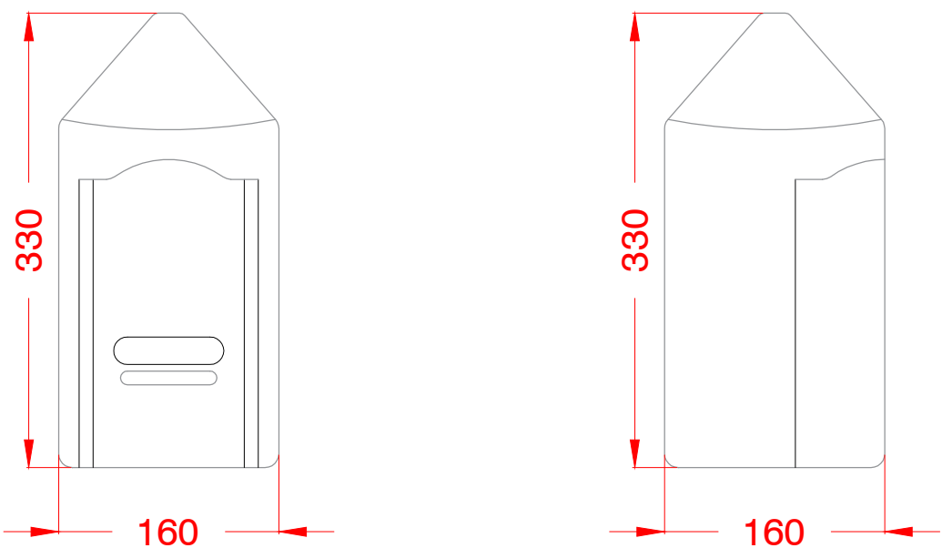
BAT BOX FRONT ELEVATION Scale: 1:5
